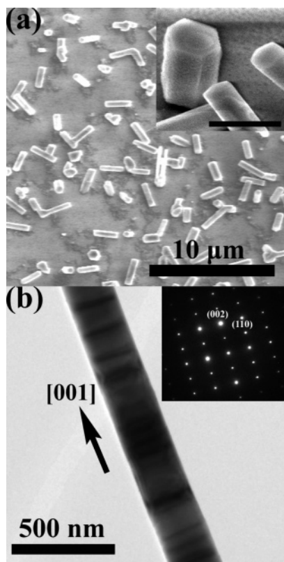
Figure 4. (a) Representative SEM image of \text{Fe}_5\text{Si}_3 nanorods. The inset shows hexagonal cross-section of the nanorods. Scale bar is 1 \mu\text{m} . (b) Representative TEM image and SAED pattern of \text{Fe}_5\text{Si}_3 nanorod. The SAED pattern is indexed for a hexagonal \text{Fe}_5\text{Si}_3 nanorod down the [110] zone axis, which elucidates the single-crystalline nature of the nanorods. The arrow indicates [001] growth direction of the nanorod. No thick silica layer on the surface could be observed in these nanorods.
